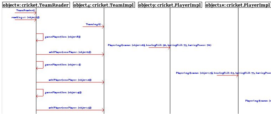
Figure 3: An example of a sequence diagram visualisation for a tiny program consisting of seven events. While sequence diagrams are useful, they become unwieldy when the execution trace contains many thousands of events.
