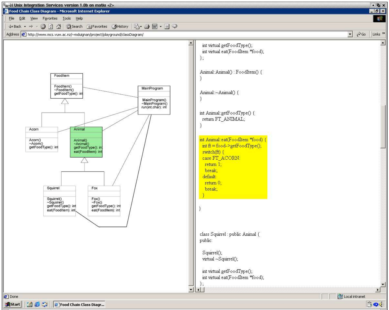
Figure 8: A SVG interactive class diagram generated by Blur (a visualisation tool) from a PAL program trace document. When the user places the mouse over a piece of code in the right hand side frame, the left hand side highlights the appropriate class or method in the UML class diagram.
