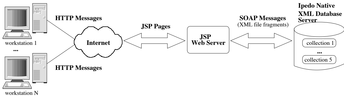
Figure 3: The XDSE architecture is based on the client/server model. The web interface communicates with a JSP web-server which sends and receives SOAP messages from the Ipedo Native XML Database. The Ipedo Native XML Database stores program trace documents in program trace collections.
