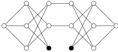
Figure 1: Fixing gadget for r = 3 .
