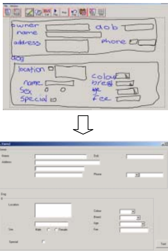
Figure 1 FreeForm Sketch to Visual Basic Form
