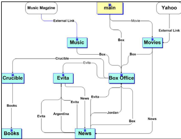
Figure 2: A simplified example of website graph
