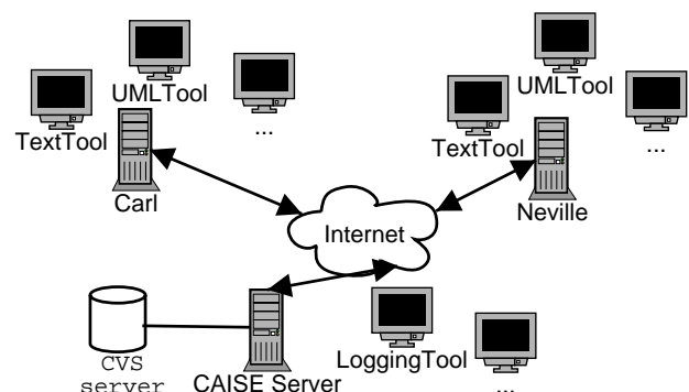
Figure 1: Collaborative software engineering
