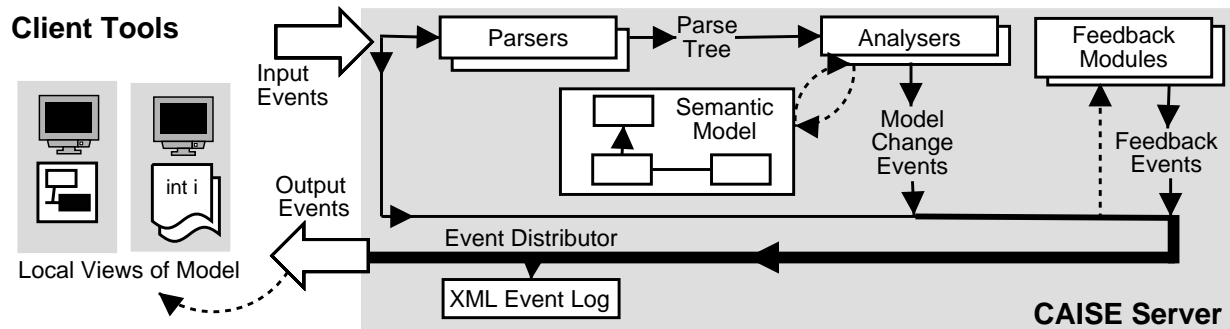
Figure 2: Event propagation in the CAISE architecture
