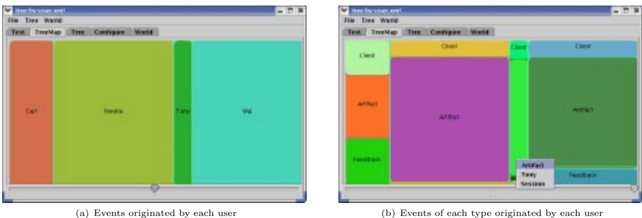
Figure 6: Treemaps showing events in a CAISE session
