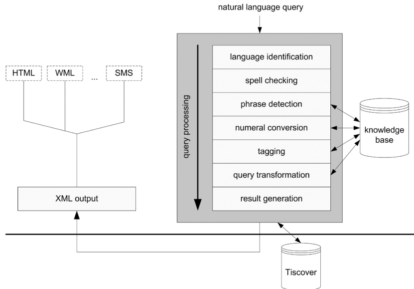
Figure 1: Software Architecture
