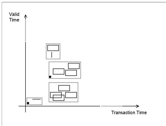
Figure 9: MBR for POINT approach
