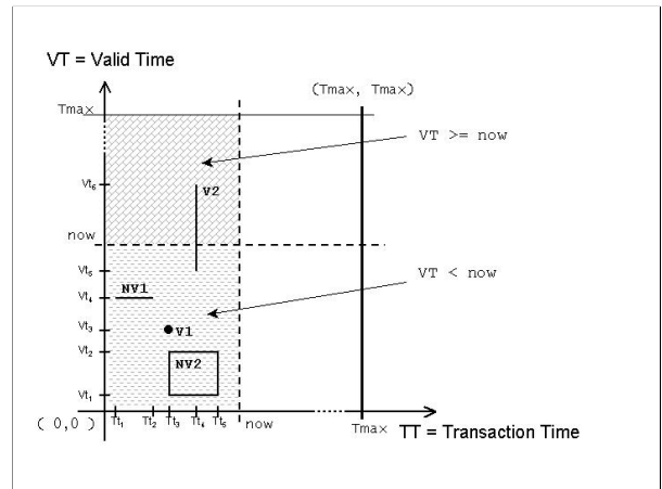
Figure 3: Query 1: Spatial POINT approach
