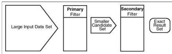
Figure 10: Oracle Spatial: Query Model
