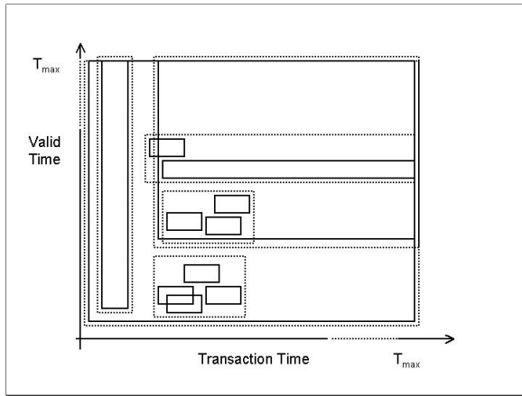
Figure 8: MBR for MAX approach
