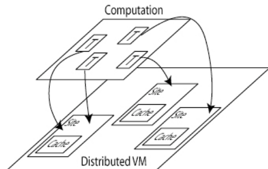
Figure 1 - ProcessBase Computational Model
